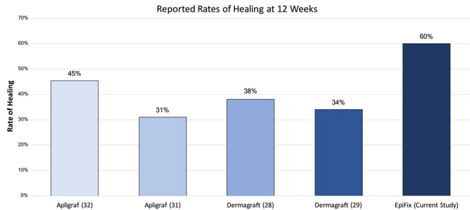
Figure 2 Comparison of 12-week healing rates reported in published randomised trials using EpiFix (current study), Apligraf (31,32) or Dermagraft (28,29) as a treatment for VLUs.
