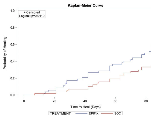
Figure 1 A Kaplan–Meier plot of time to heal within 12 weeks by study group.
